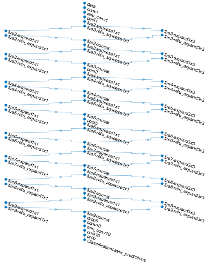
Figure 1. The Structure Of A Neural Network Of The Squeezenet Type
