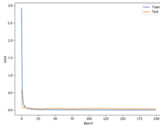
Figure 9. The Diagram Of Recognition Losses Versus The Number Of Training Periods
