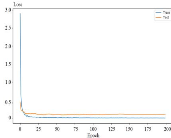
Fig. 11 Graphs Of The Dependence Of Losses On The Number Of Training Eras When Exposed To Noise
