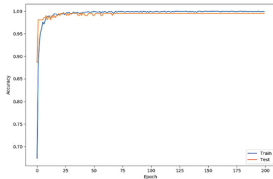
Figure 8. The Diagram Of Recognition Accuracy Versus The Number Of Training Periods
