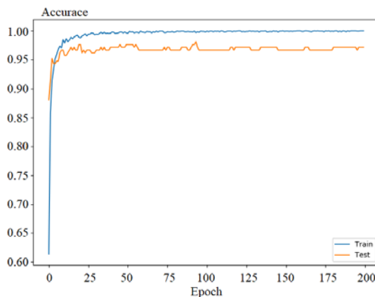
Fig. 10 Graphs Of The Dependence Of Recognition Accuracy On The Number Of Training Eras When Exposed To Noise
