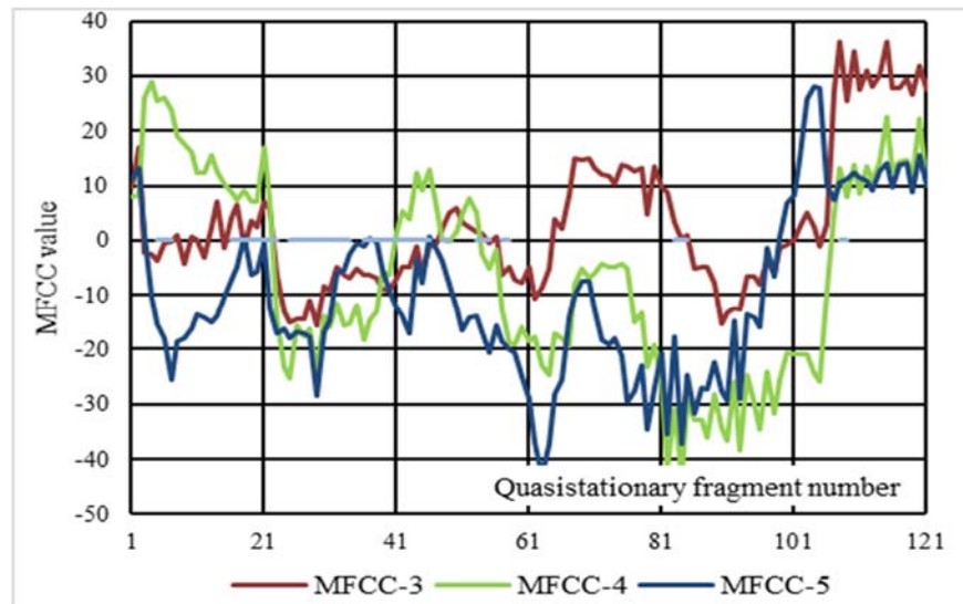
Fig. 4. Graphs Of MFCC Values when Scoring The Text "Say The Word Back"
